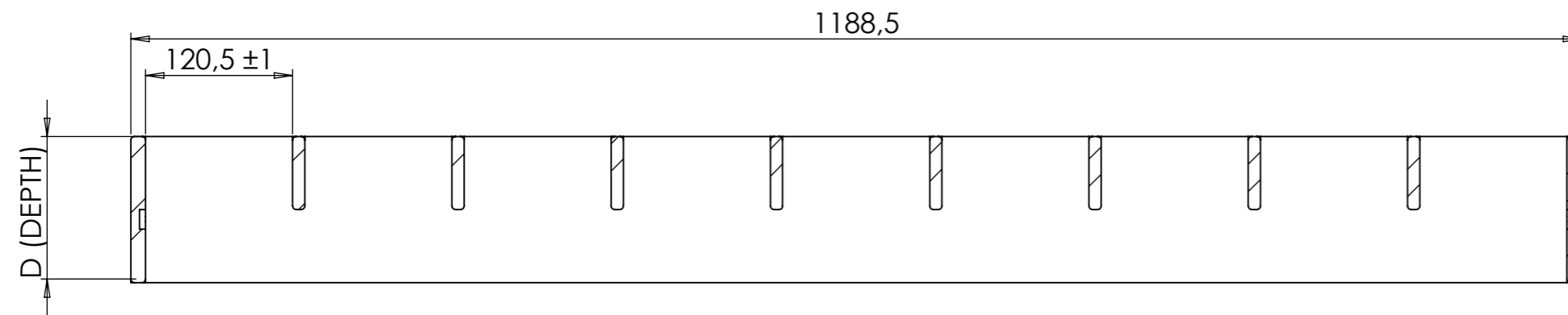
SECTION B-B
