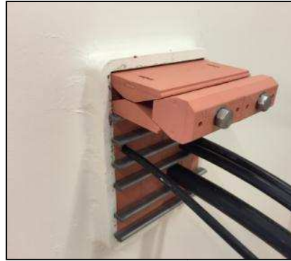
Insert the PTG on top of the final stay plate.
