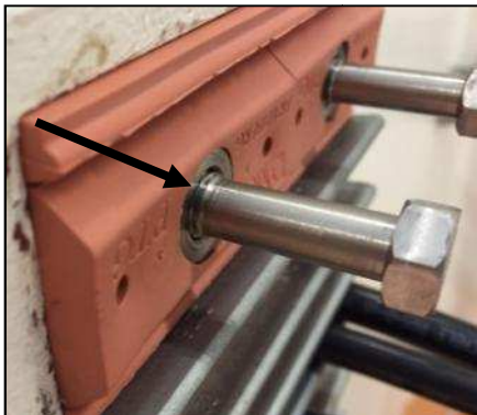
Tighten the bolts to the bottom or until the thread clearly is visible as per the picture.
